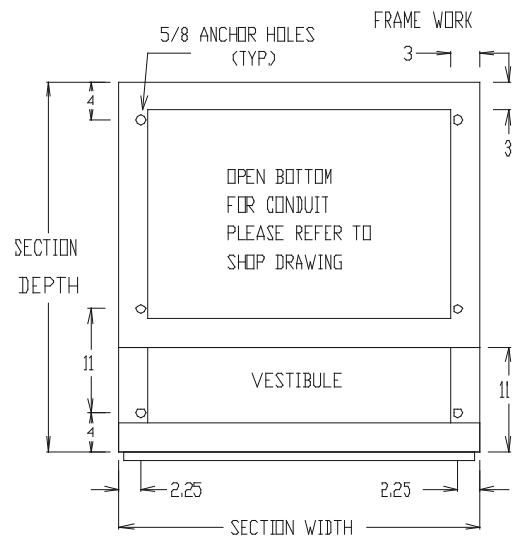
NEMA 3R - BASE DETAIL OUTDOOR
