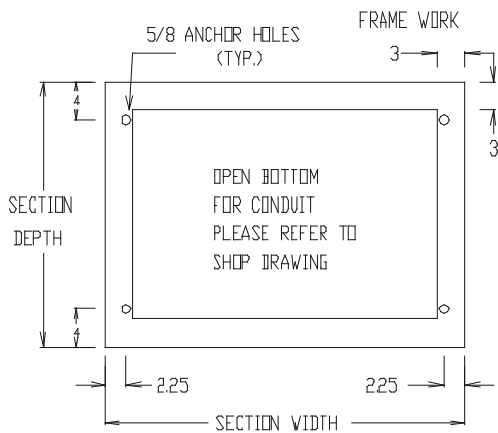
NEMA 1 - BASE DETAIL INDOOR
