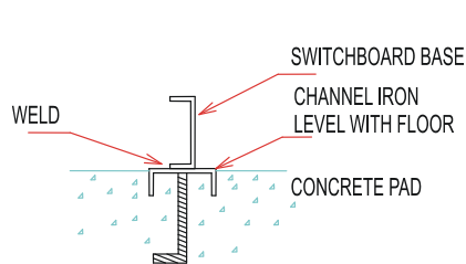
Suggested method of installing floor channels by installing contractor
