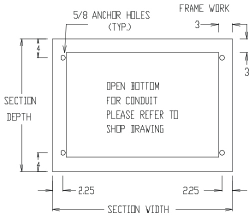
NEMA 1 - BASE DETAIL INDOOR
