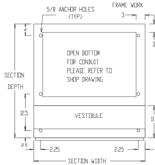
NEMA 3R - BASE DETAIL OUTDOOR
