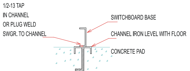
Suggested method of installing floor channels by installing contractor
